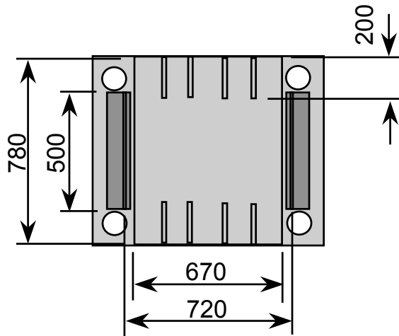
Larger heating platen (670x780 mm)
