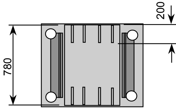
Longer heating platen (560x780 mm)
